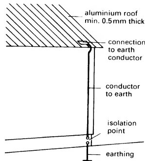
④ Aluminium roof decking used as a lightning conductor
